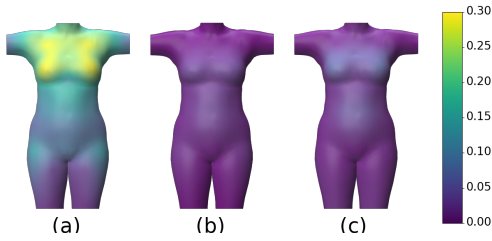
Figure 7: Norm of covariance of elasticity parameters on the train subjects: (a) optimized independently, (b) with our method, (c) with L^2 regularization.
