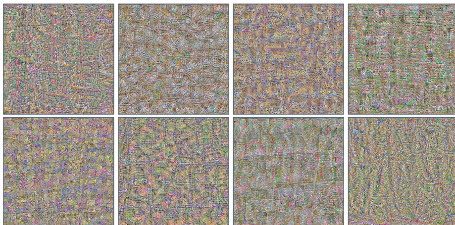
Figure 34. Visualization of some filters in the twelfth layer of our model.
